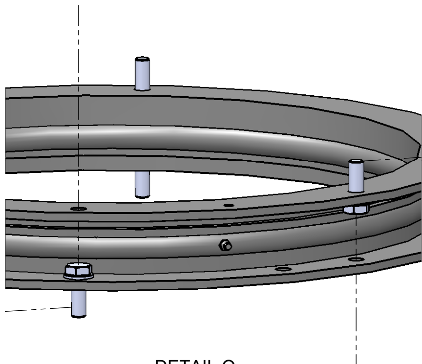
DETAIL O SCALE 1 : 3
