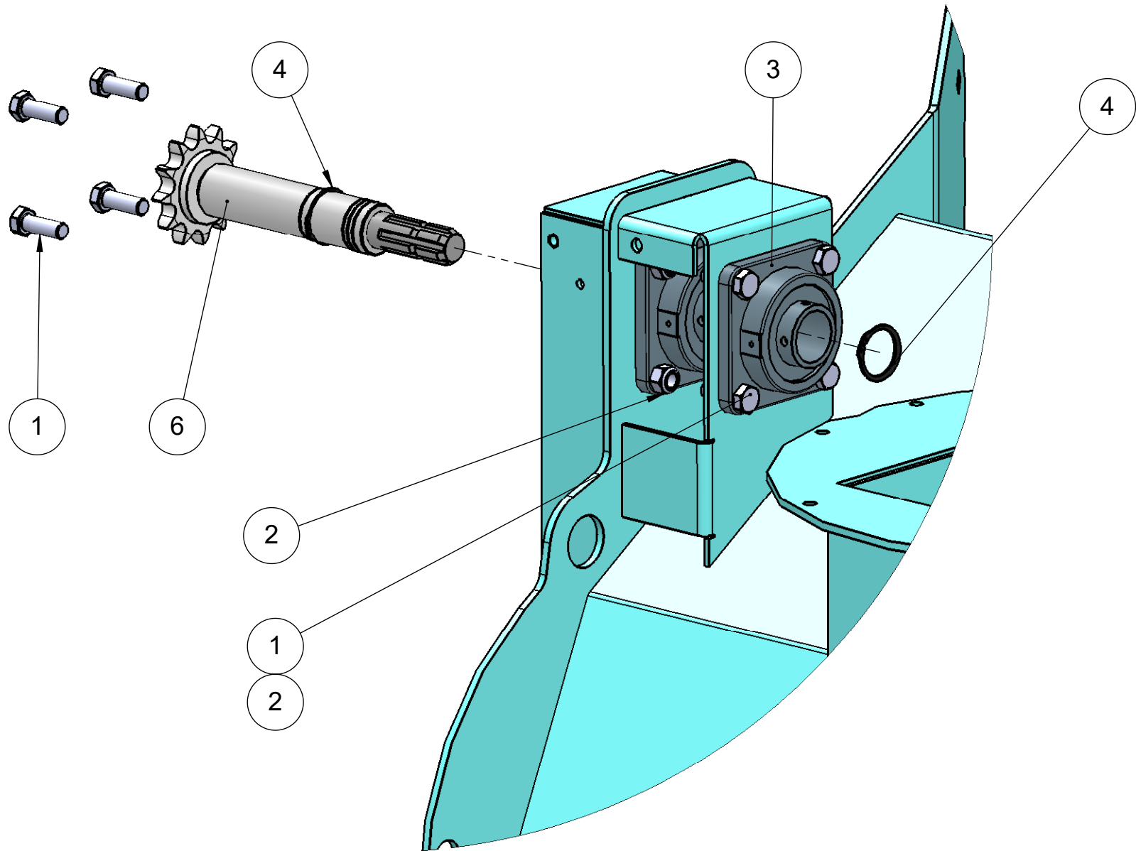
DETAIL K SCALE 1 : 5
